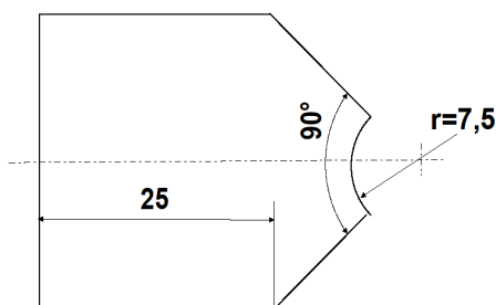
TEMPLATE FOR NOSE-/SPINNER-RADIUS
